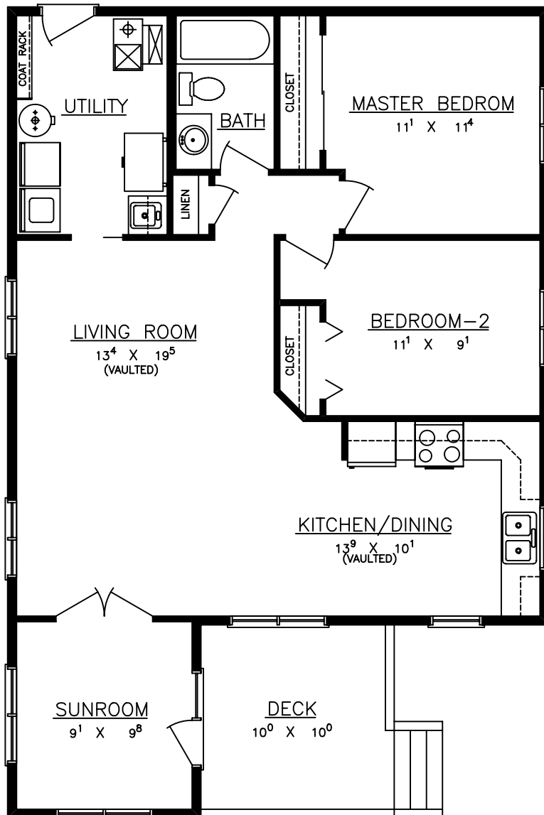
FLOOR PLAN
